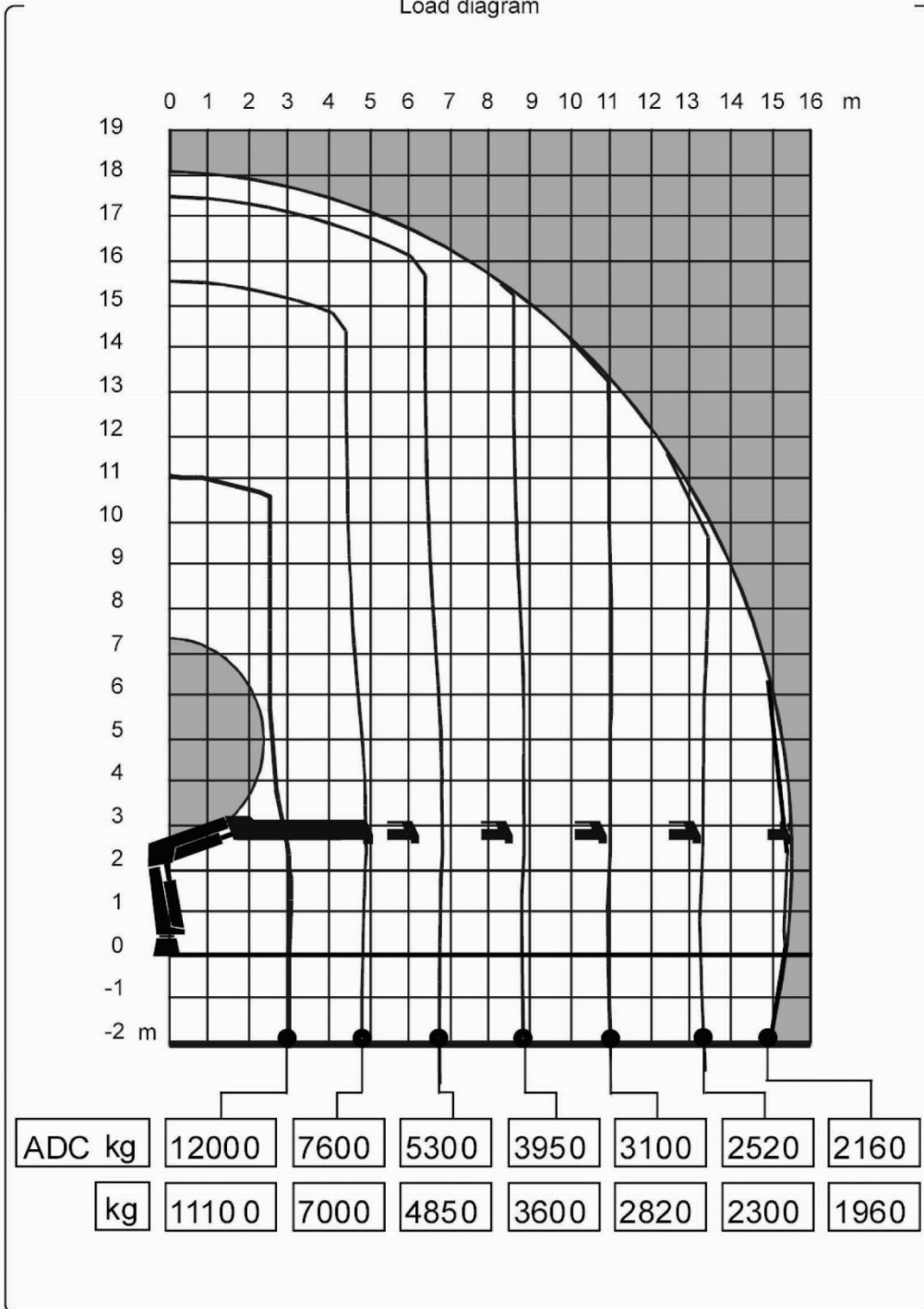
Load diagram
