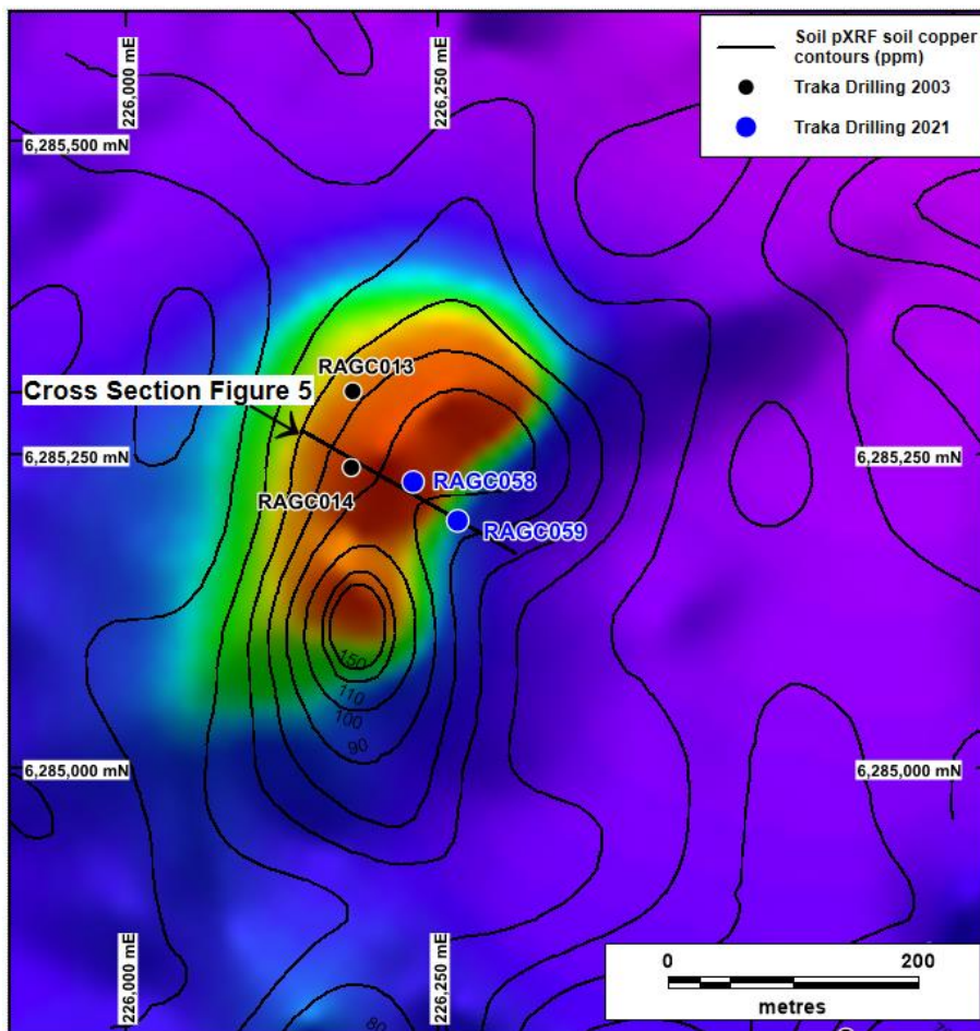
Figure 2. Aeromagnetic image plan view of the Revelation Prospect showing the coincident bulls-eye (red colour) magnetic anomaly with pXRF copper soil anomaly (black contours). The new drill holes (blue dots) and Traka's old drill holes (black dots) are shown.
