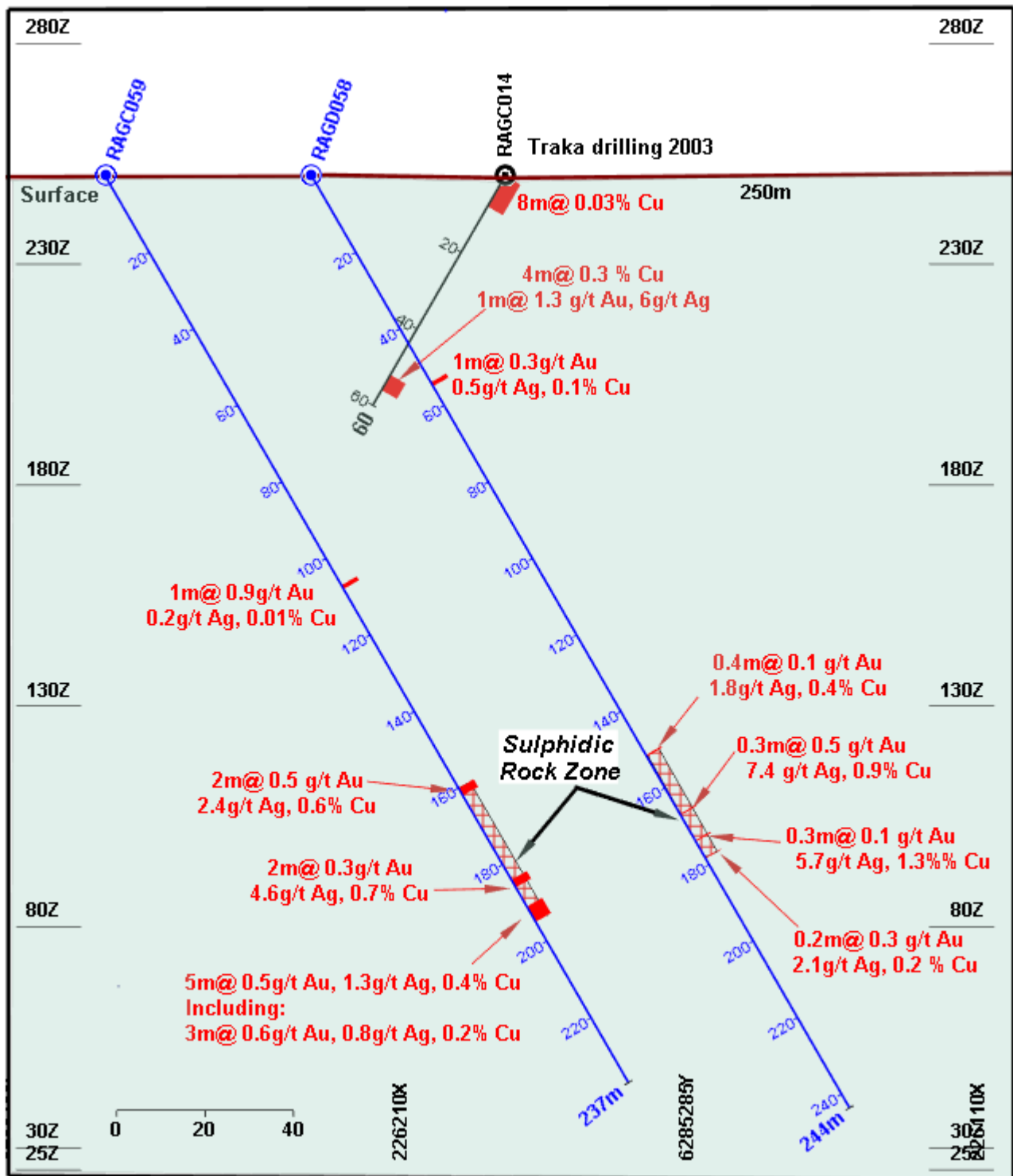
Figure 1. Cross-section through the Revelation Prospect showing drillhole RAGC058 and RAGC059 and Traka's drillhole in 2003
